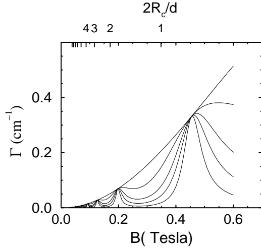
FIG. 1. Absorption coefficient \Gamma of SAW as a function of the magnetic field for the transverse orientation, \mathbf{p} \perp \mathbf{q} and the following values of the parameters: density n_e = 1 \cdot 10^{11} \text{ cm}^{-2} , \omega = 2\pi \cdot 300 \text{ MHz} , \tau = 150 \text{ ps} , d = 300 \text{ nm} . The strength of the grating \eta is equal to (from the top to the bottom): 0 (no grating), 0.01, 0.02, 0.03, and 0.05.
